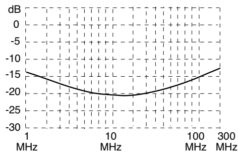
Typical Common Mode Attenuation
